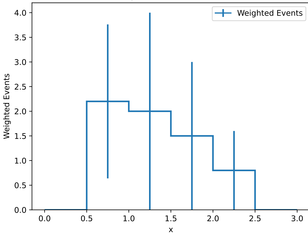
Weighted Unbinned Data
