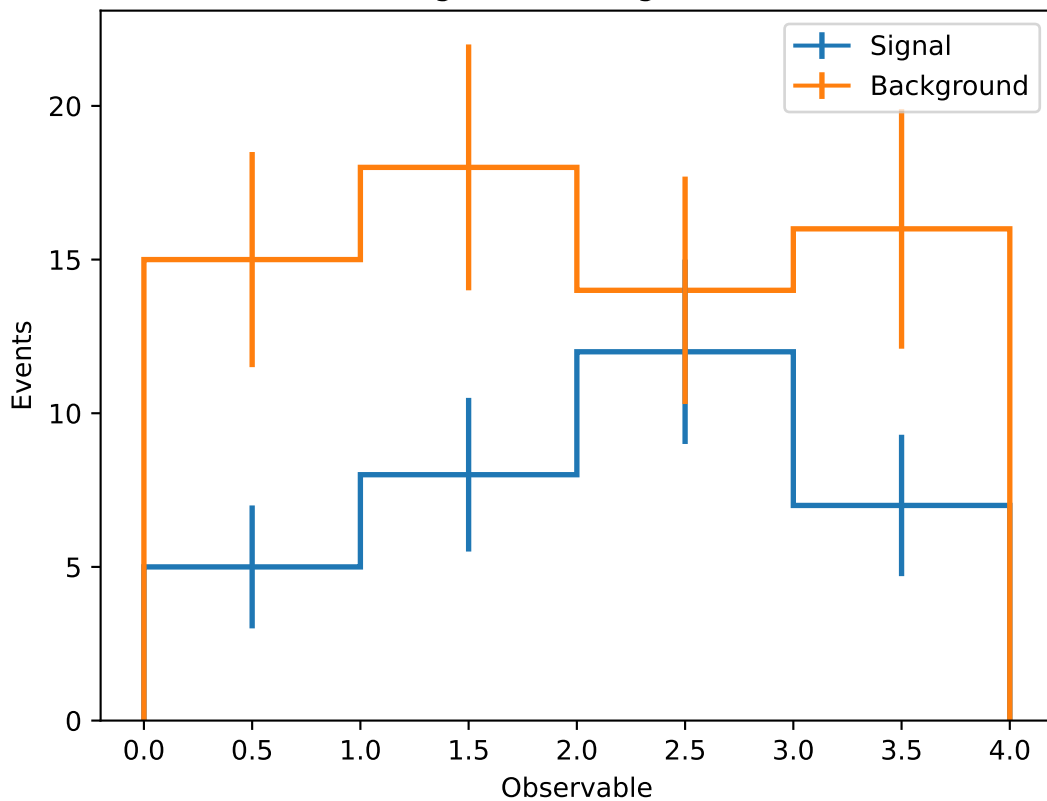
Signal vs Background
