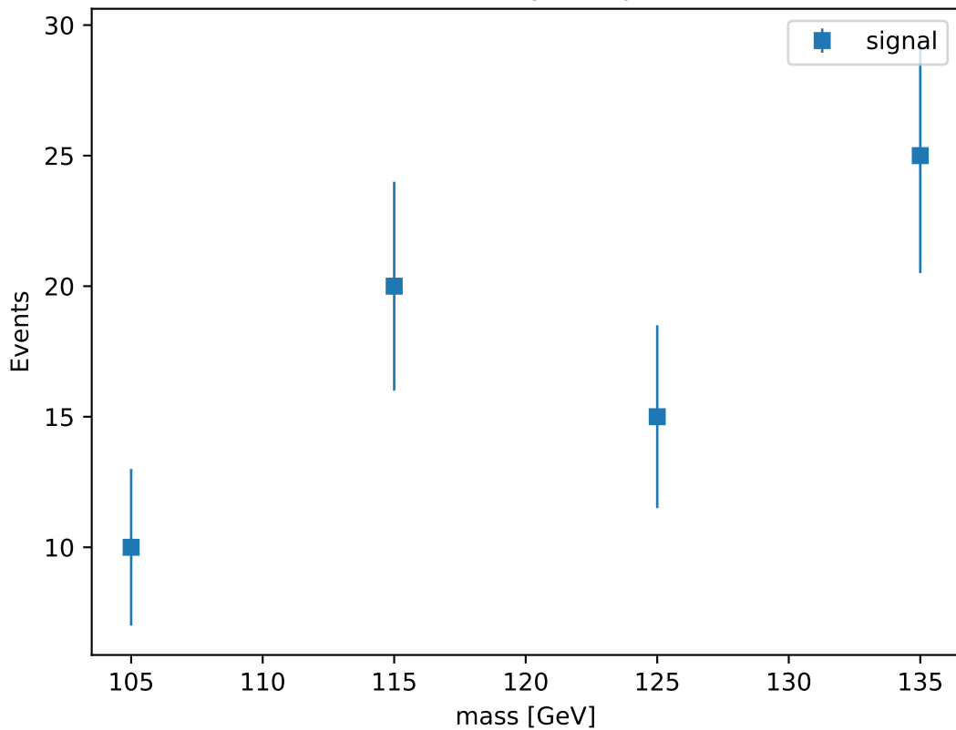
HistFactory Sample
