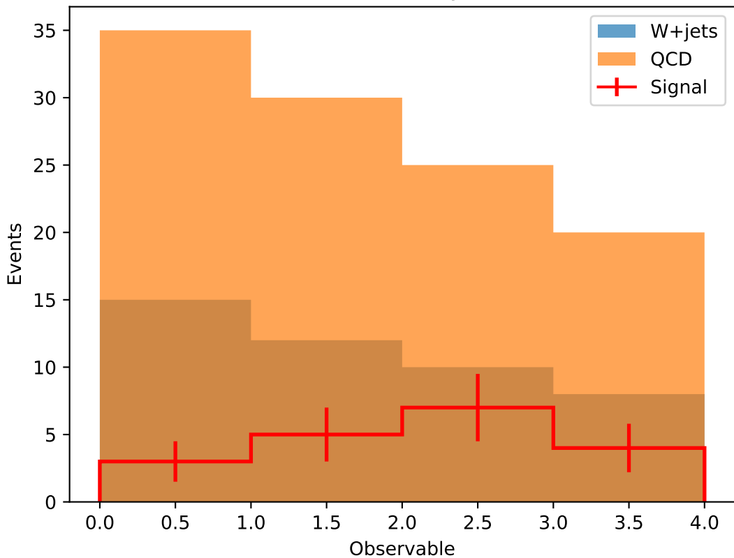
Stacked HistFactory Channel
